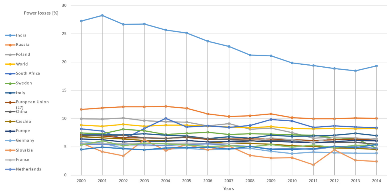
Fig. 2. Electricity transmission and distribution power losses [12]
