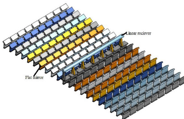
Fig. 4. Schematic diagram of linear Fresnel system
