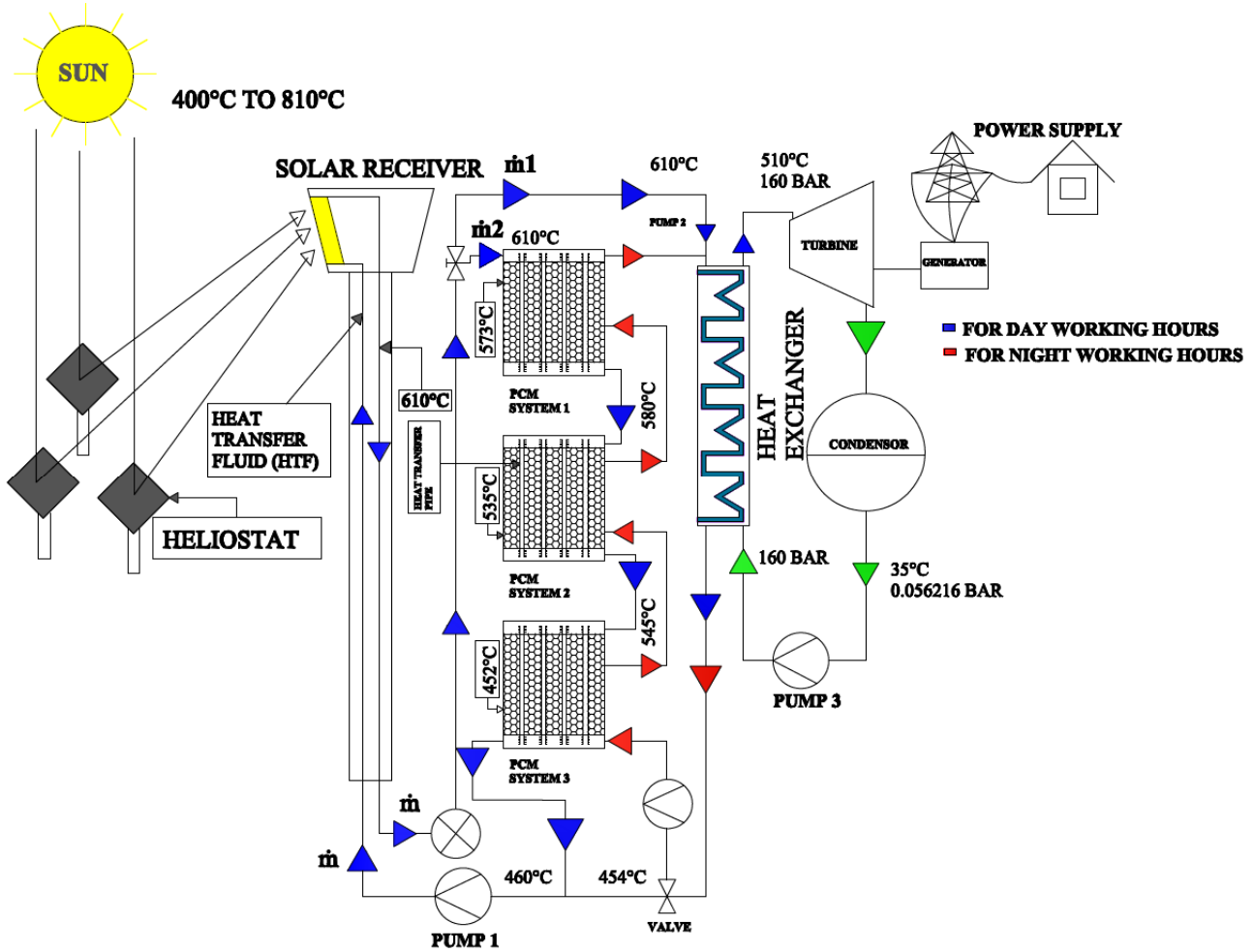
Fig. 8. A schematic representation of a typical layout of a solar thermal power plant (STPP)
