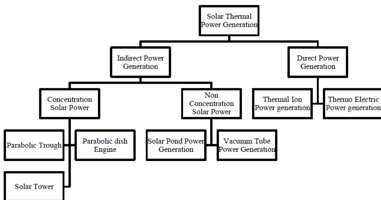
Fig. 1. Classification of solar thermal power generation
