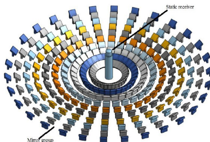
Fig. 3. Schematic diagram of power tower system
