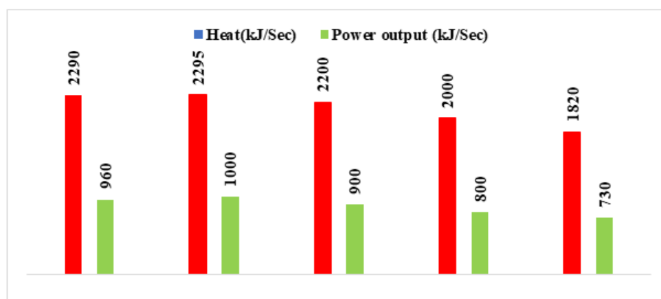
Fig. 10. Rise in power output with respect to the increase in heat input
