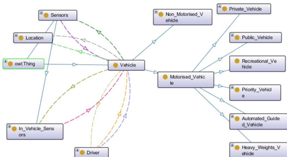
Fig. 6. Class "Vehicle" and its relations.
