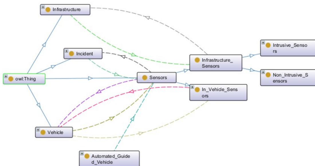
Fig. 5. Class "Sensor" and its relations.
